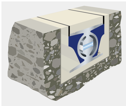
Cross-cut of installed Lineas WIM sensor
