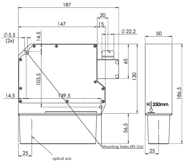
Fig. 3: Dimensions of Correvit® S-HR sensor with 90° connector
