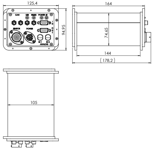
Fig. 2: Dimensions of Correvit® S-HR electronics
