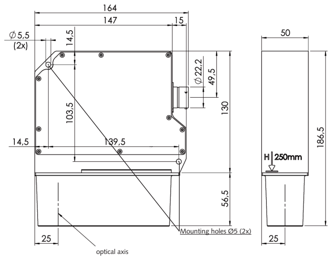
Fig. 1: Dimensions of Correvit® S-HR sensor
